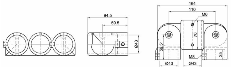
Kreuz-Gelenkverbinder, 1-schalig Cross-joint connector, 1-shell
