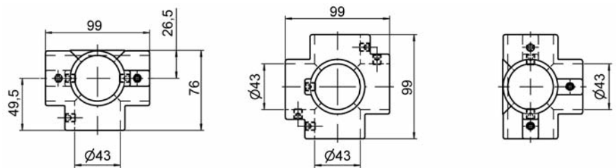
Kreuzverbinder 5-fach, 1-schalig Cross connector 5 end, 1-shell
